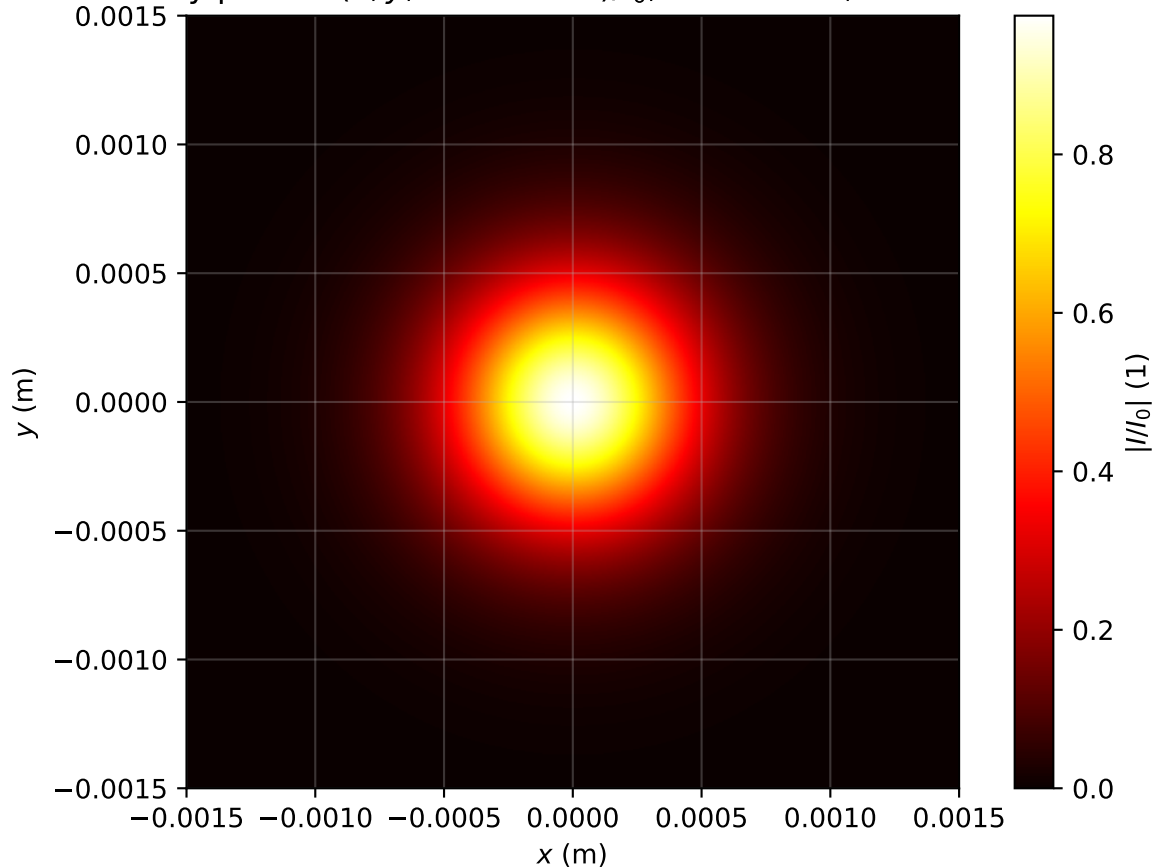
Intensity profile I(x, y, z = 1.433m)/I_0 , P_{in}=0.5P_{cr} , artificial time
